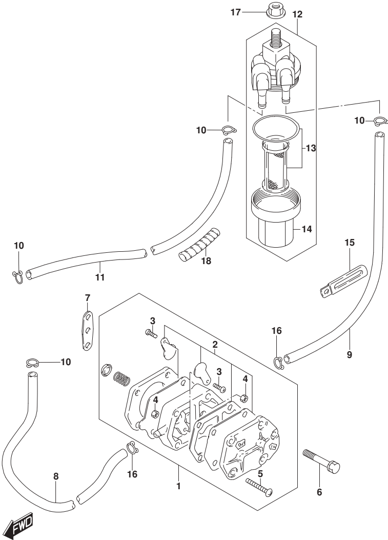
DT25_30_P40_016_146B FUEL PUMP
