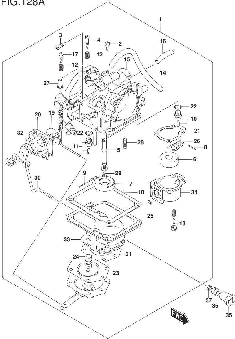
DT25_30_P40_016_128A CARBURETOR
