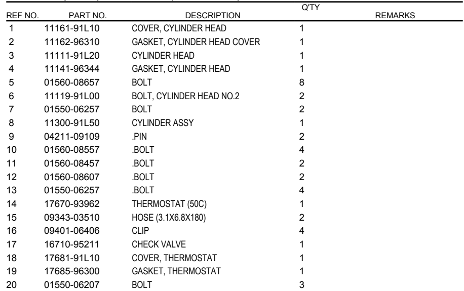
FIG.112C (1-B-4) CYLINDER (DT30R P40)
