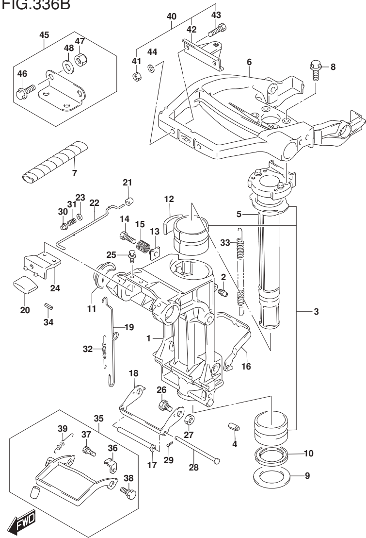
DT25_30_P40_016_336B SWIVEL BRACKET
