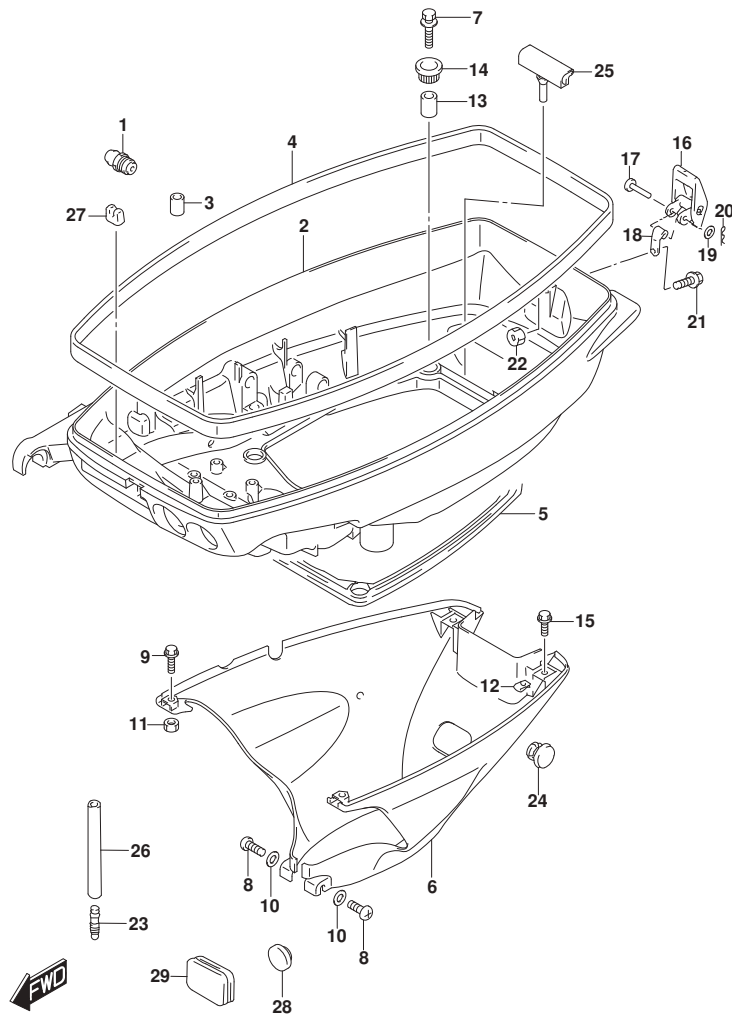
DT25_30_P40_016_413C UNDER COVER
