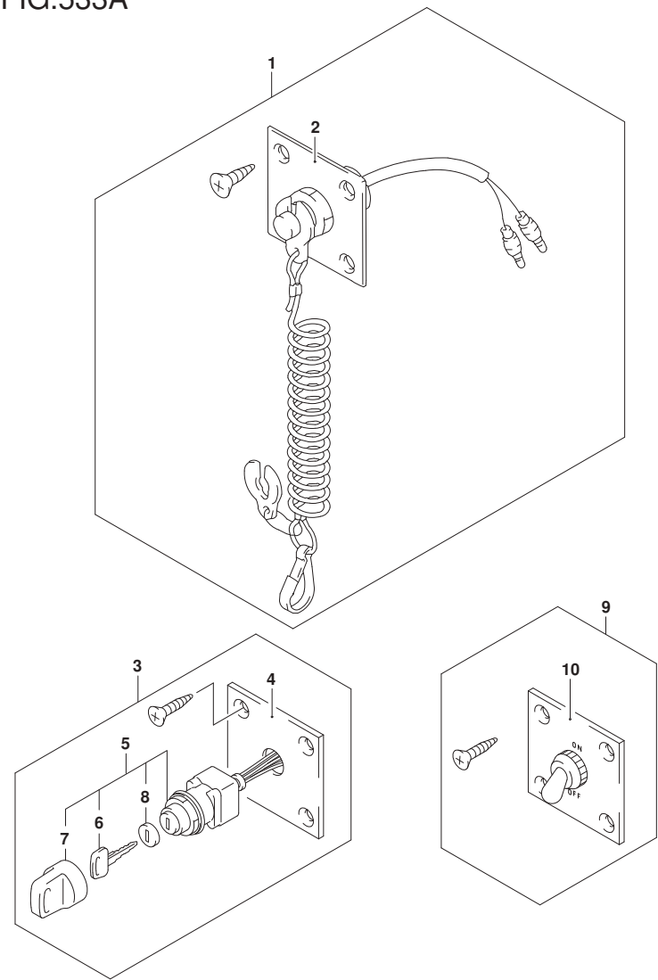
DT25_30_P40_016_533A OPT:SWITCH PANEL
