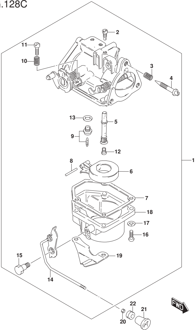
DT25_30_P40_016_128C CARBURETOR
